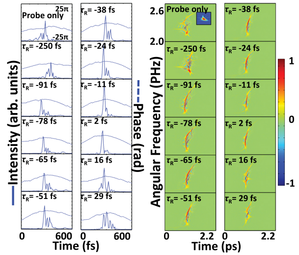
FIG. 2. (Color online) Left side: envelope I(t) and phase \Phi(t) plots of the probe pulse exiting the two-pulse filament. The shortest pulse, with 21-fs FWHM, occurs in the range of -11 \text{ fs} < t_R < 2 \text{ fs} . For all probe delays, \partial^2 \Phi / \partial t^2 < 0 throughout the pulse envelope, indicating a dominant redshift to blueshift. Right side: Wigner plots corresponding to the plots on the left. The Wigner plot for the prefilamenting probe alone is shown highlighted in the upper left panel.
