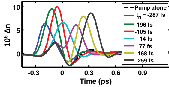
FIG. 3. (Color online) Density-matrix simulation of the self-consistent refractive index change experienced by a variably delayed 2 \times 10^{13} W/cm 2 100-fs probe pulse perpendicularly polarized with respect to a similar pump pulse. The probe delays t_R are relative to the zero crossing of the pump-induced air rotational revival near 8.3 ps, shown as the dashed curve.
